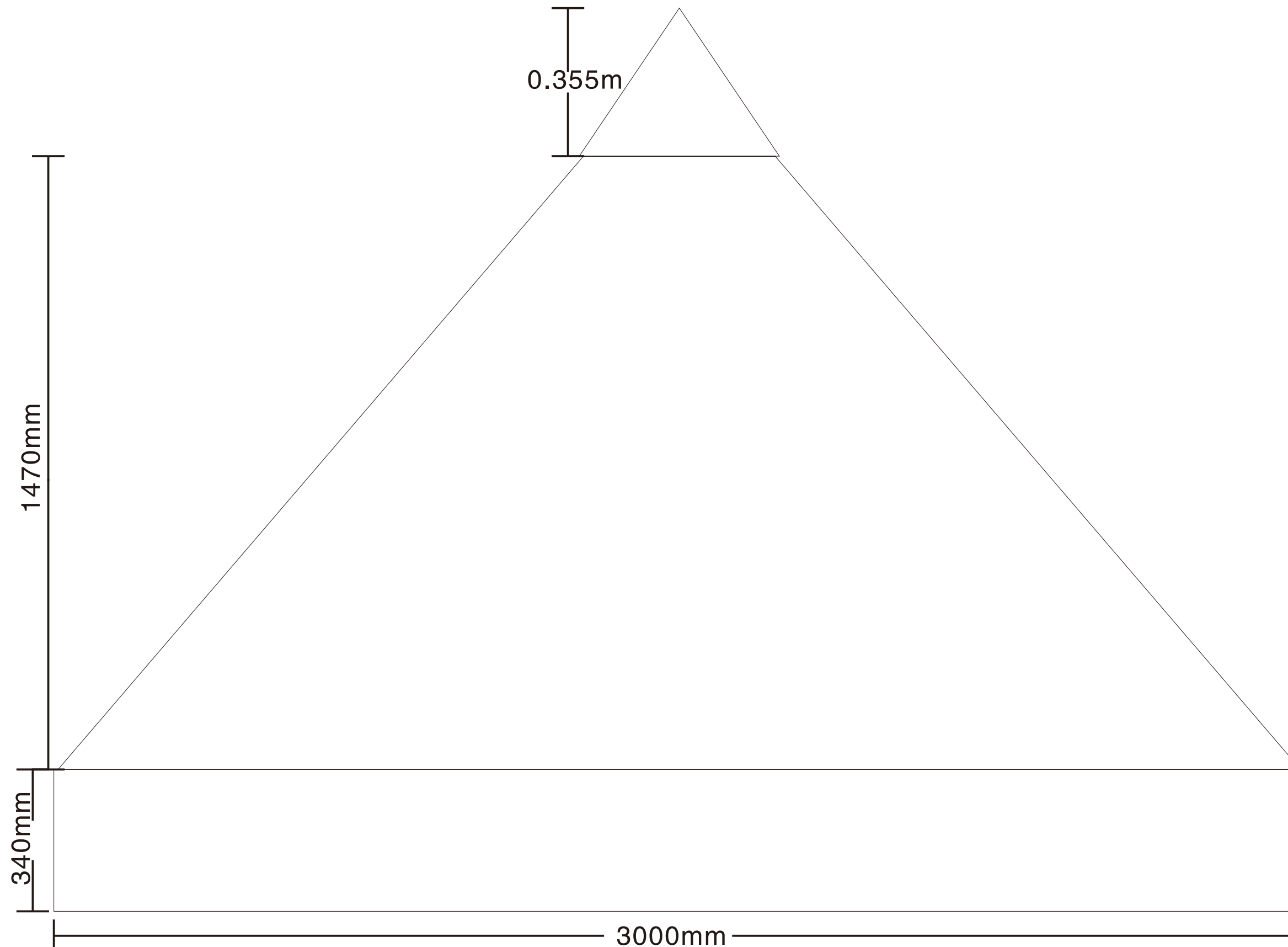
RIGHT VALANCE PANEL
