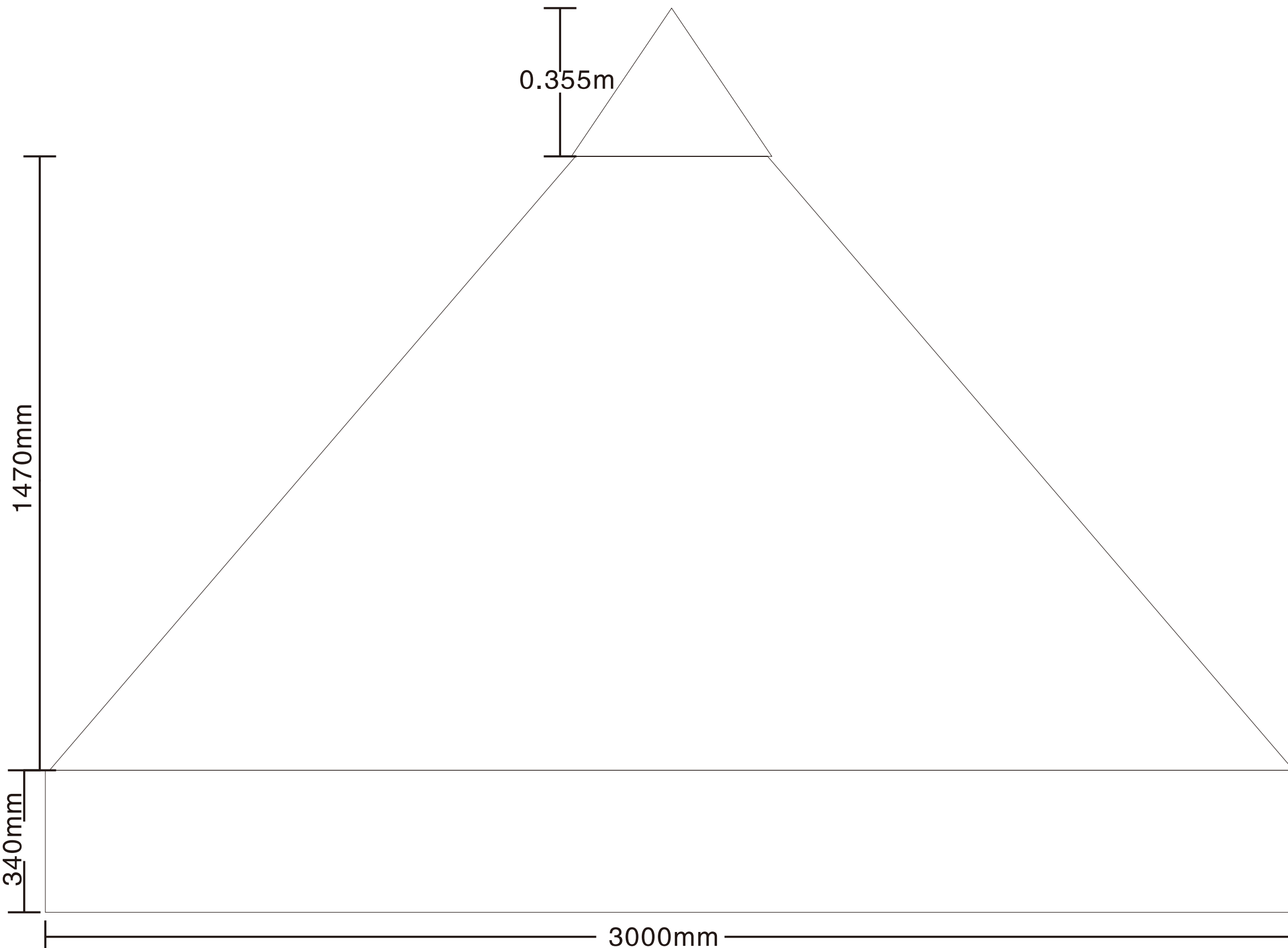
BACK VALANCE PANEL
