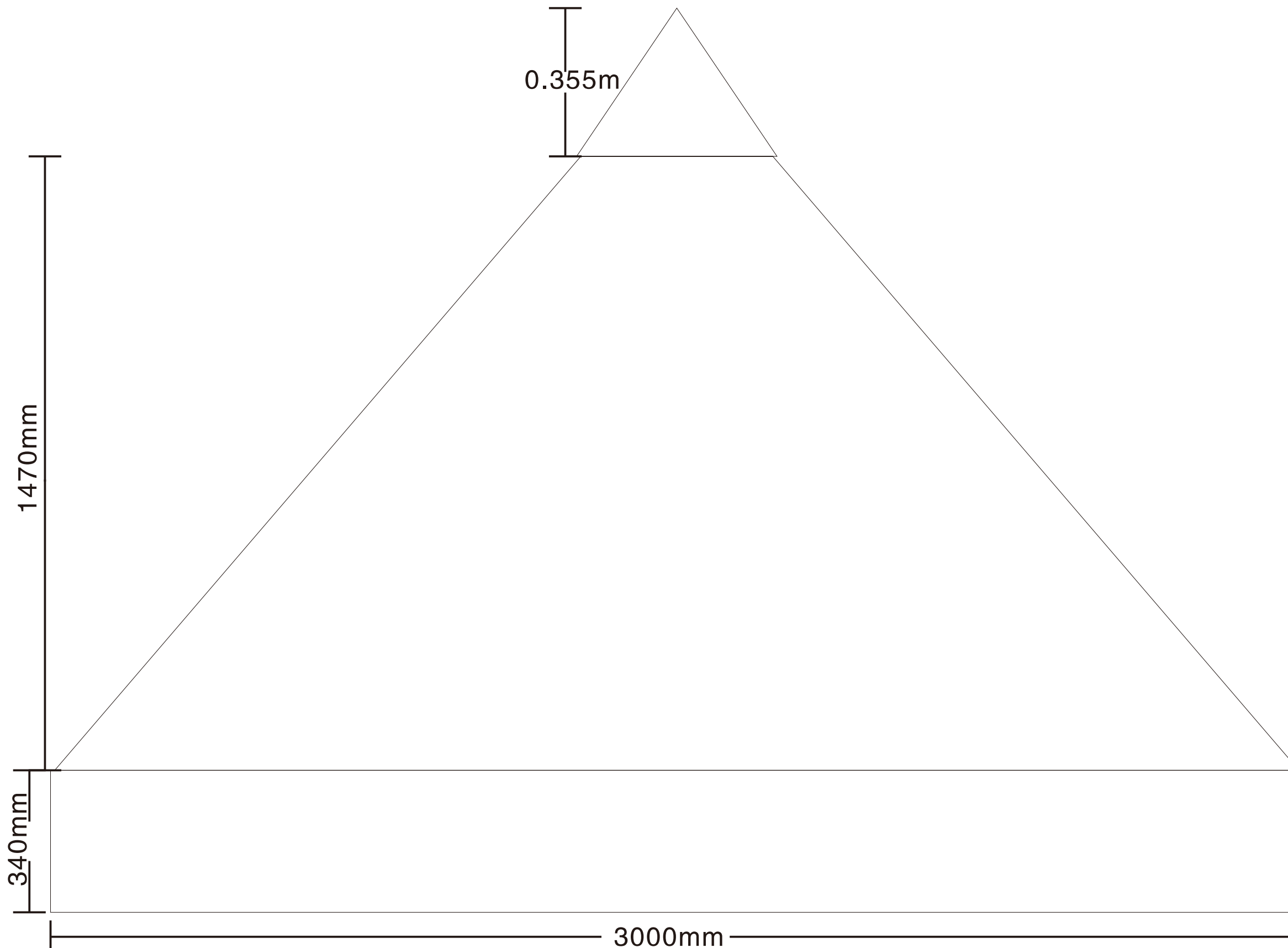
FRONT VALANCE PANEL
