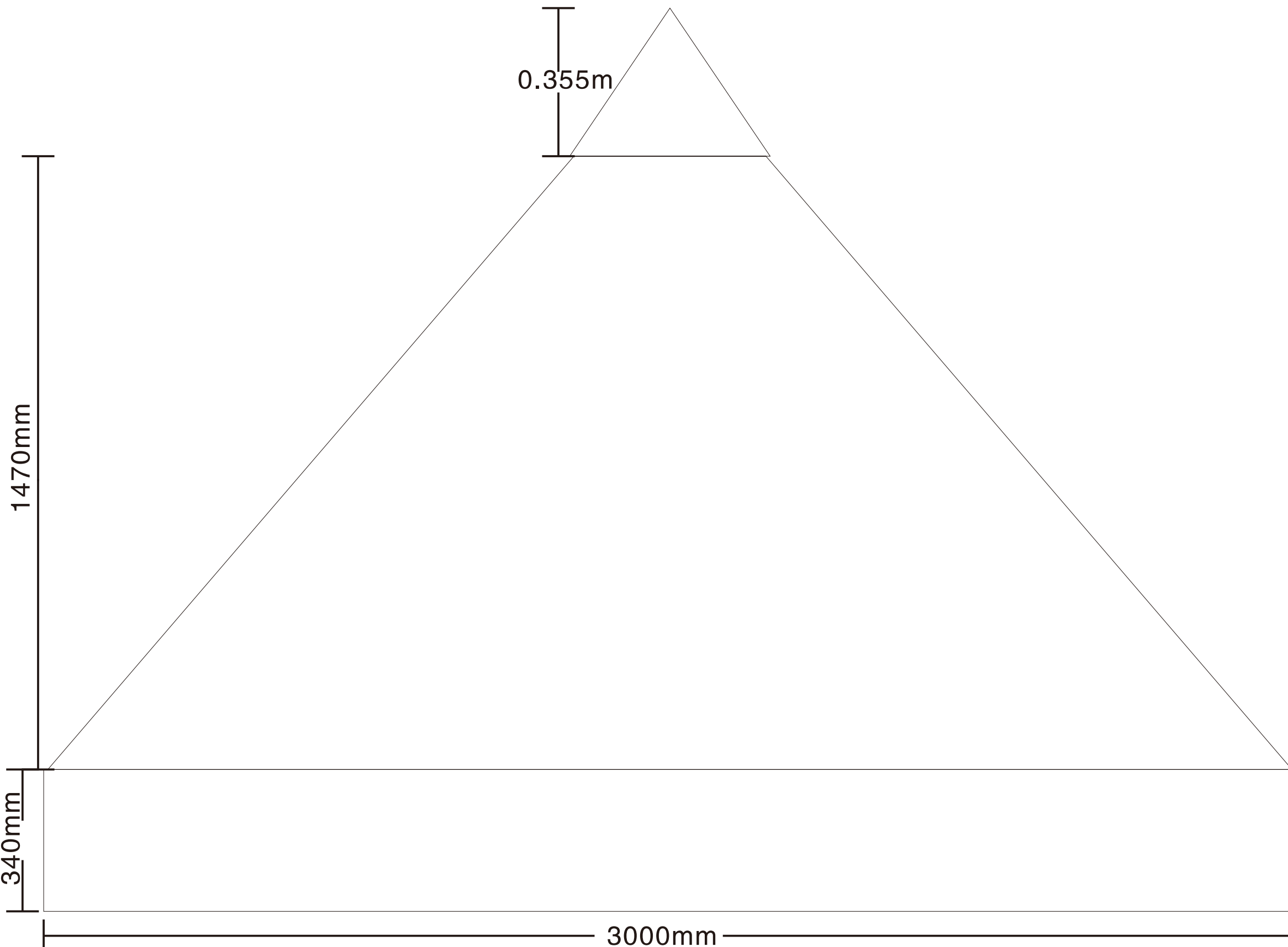
LEFT VALANCE PANEL
